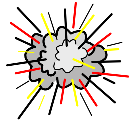
Big Bang
