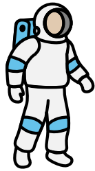
Astronaut
